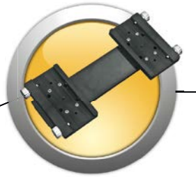
3" LODUAL double mounting plate balancing design, with 2 pcs. 3" dovetail clamps #1452085 for mounting of two telescopes. Maximum Center-to-center distance 27 cm #1452105
